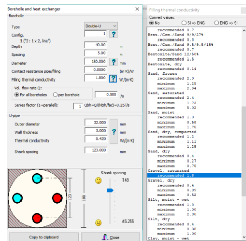
Fig. 5. EED software vertical boreholes and filling material properties
